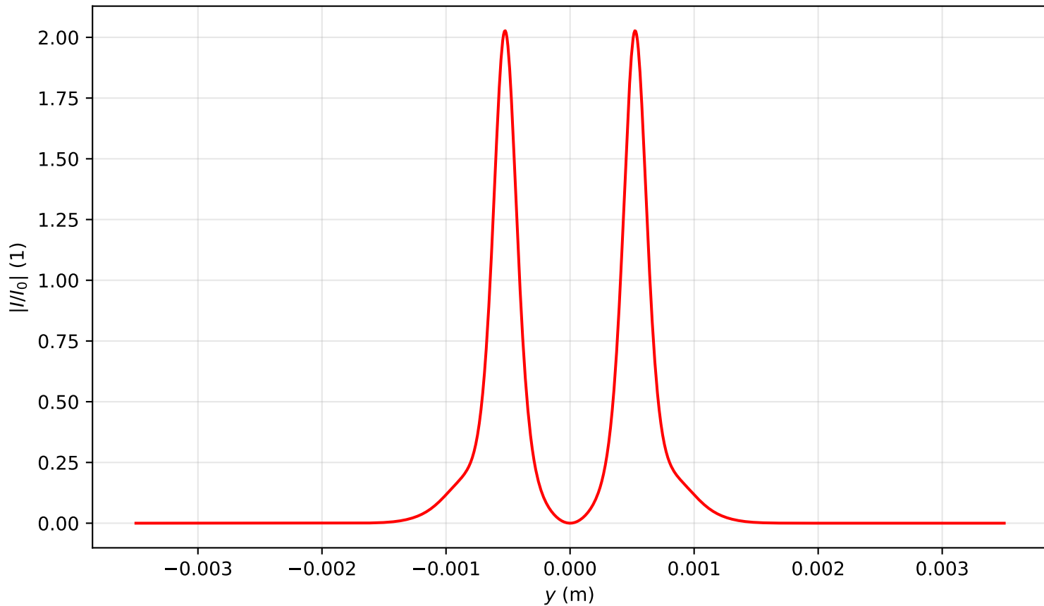
Intensity profile I(x=0, y, z=0.478)/I_0 , P_{in}=9.0P_{cr} , artificial time
